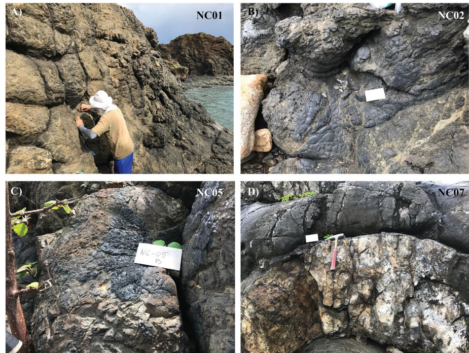
Figure 2. Field photographs showing the sampling of the SBGs in pillow lava margins from the Nicoya Peninsula and Murciélago Islands (Costa Rica). SBG, submarine basaltic glass.
